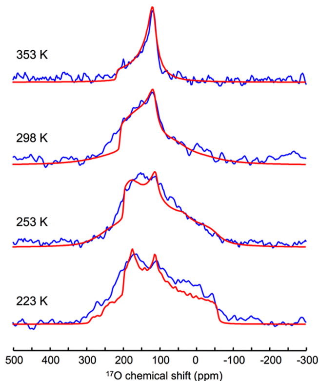
Figure 3. Experimental (blue) and simulated (red) solid-state ^{17}\text{O} NMR spectra of [\text{K}_2(\text{DMF})_2][\text{CO}^{17}\text{O}_2\text{CmBDCA-5t-H}_6] at different temperatures. All spectra were recorded at 14.1 T.
