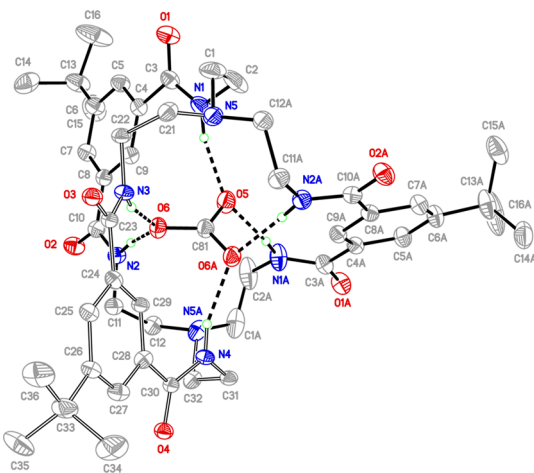
Figure 2. Solid-state structure of [(\text{TBA})_2][\text{CO}_3\text{CmBDCA-5t-H}_6] with thermal ellipsoids plotted at the 50% probability level. Counter cations, solvent, and all hydrogen atoms are omitted for clarity except for the N–H carboxamide protons engaged in hydrogen bonding with the carbonate anion. Selected interatomic distances (Å) and angles (deg): C81–O(carbonate) 1.291(avg), N5–N5A 7.687(2), N1–O5 2.739, N2–O6 2.754(2), N3–O6 2.72(2), N4–O6A 2.79(1), O5–C81–O6 120.2°, O6–C81–O6A 119.7°, C9–O6 3.151(1), C9–O5 3.257, C29–O6 3.14(1), C29–O6A 3.19(1).
