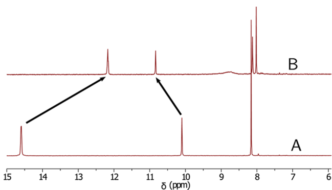
Figure 1. ^1\text{H} NMR spectra of [(\text{TBA})_2][\text{O}_2\text{CmBDCA-5t-H}_6] (A) and [(\text{TBA})_2][\text{CO}_3\text{CmBDCA-5t-H}_6] (B) in \text{DMSO-}d_6 after exposure to CO gas ( 40^\circ\text{C} , 3 h).
